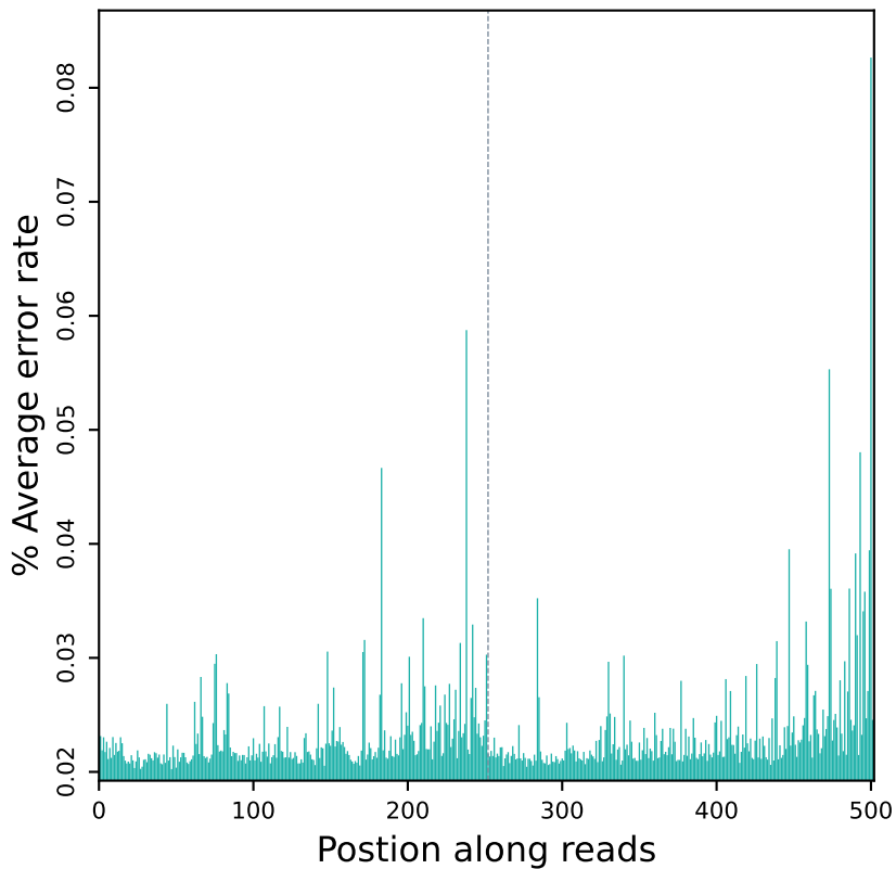
Error rate distribution along reads (R10404)
